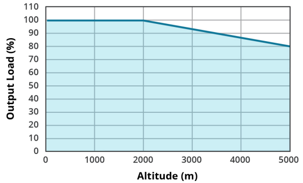
ALTITUDE DERATING CURVE
