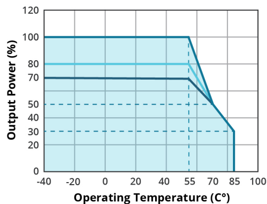
TEMPERATURE DERATING CURVE without aluminum plate (85~305 Vac, 120~430 Vdc)
