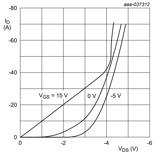
Fig. 8. Third quadrant characteristics; typical values
