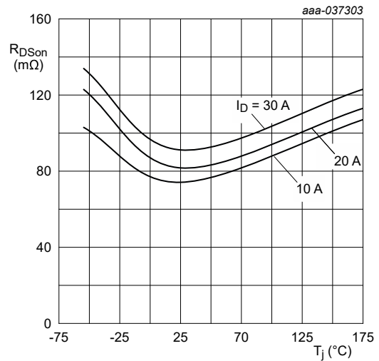
Fig. 4. Normalized drain-source on-state resistance as a function of junction temperature; typical values
