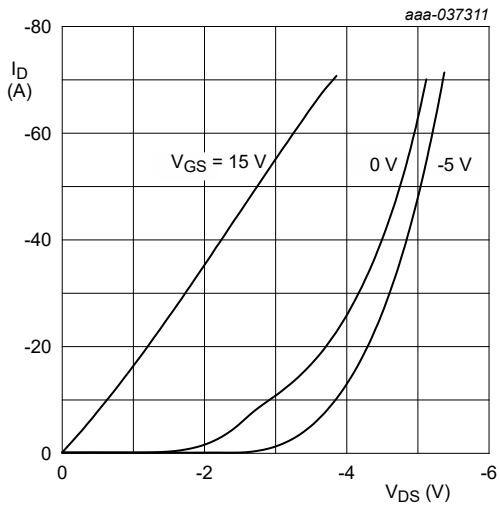
Fig. 7. Third quadrant characteristics; typical values
