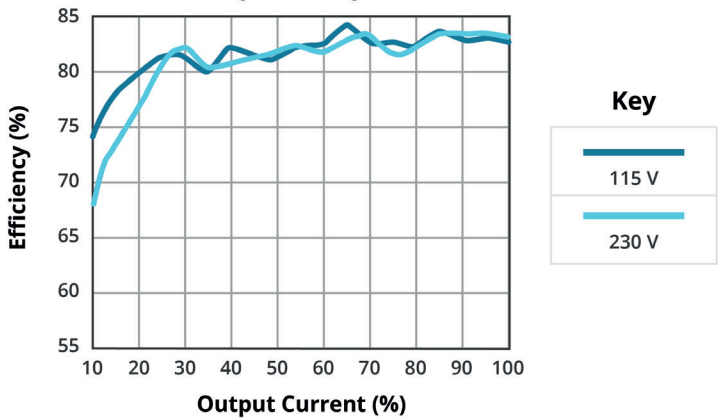
EFFICIENCY VS OUTPUT LOAD (VOF-4-24)
