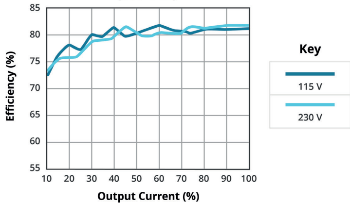
EFFICIENCY VS OUTPUT LOAD (VOF-4-12)
