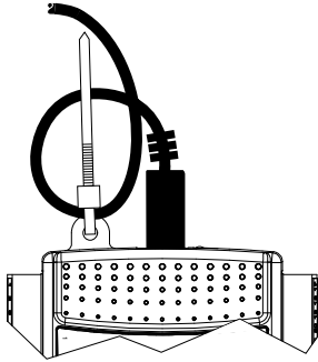
Figure 5. NI USB-6008/6009 Strain Relief
