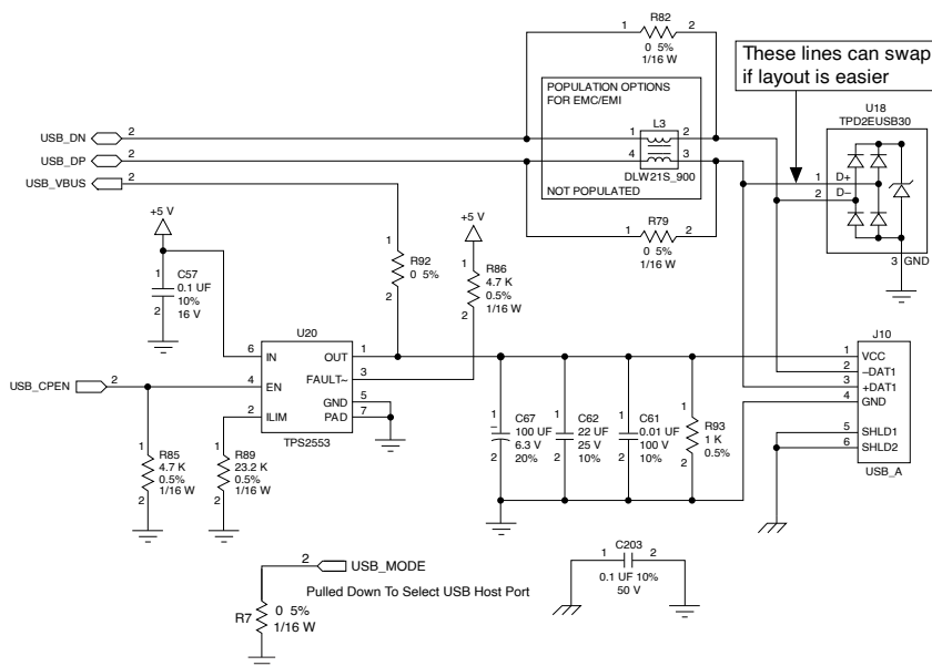
Figure 4. USB Host Reference Schematic
