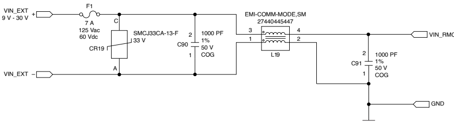
Figure 1. VIN_Filtered Reference Schematic
