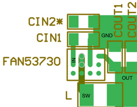
Figure 36. Layout Example
