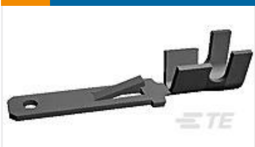
TE Part #61316-1 FF 250 TAB 22-18AWG TPBR
