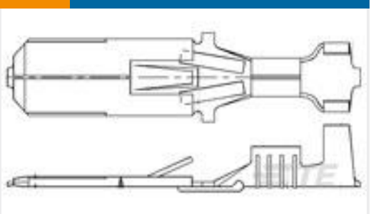
TE Part #42241-2 FF 250 TAB 18-14 AWG .032 TPBR
