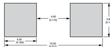
Recommended Pad Layout
