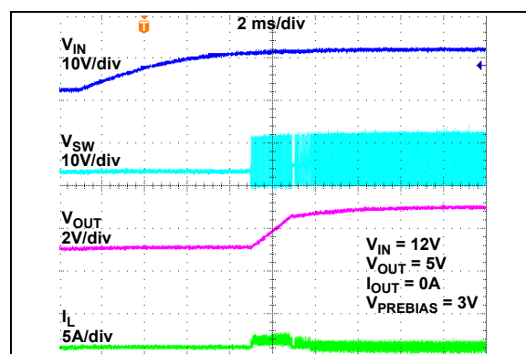
FIGURE 2-41: V_{IN} Start-up Pre-Biased Output.
