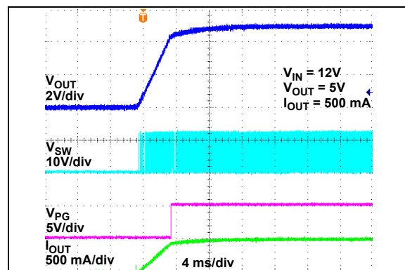
FIGURE 2-54: Recovery from Thermal Shutdown.
