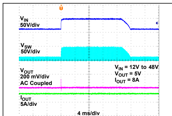
FIGURE 2-64: Line Transient Response ( V_{IN} = 12V to 48V ).
