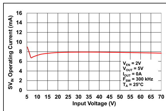
FIGURE 2-28: SV_{IN} Operating Current vs. Input Voltage.
