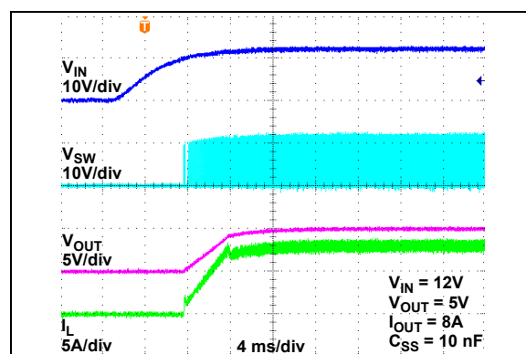
FIGURE 2-42: V_{IN} Soft Turn-On.
