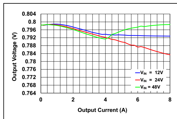
FIGURE 2-4: Output Voltage vs. Output Current ( V_{OUT} = 0.8V ).
