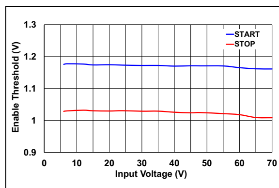
FIGURE 2-30: Enable Threshold vs. Input Voltage.
