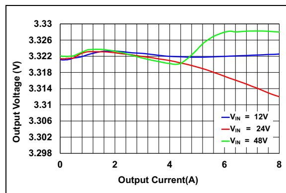
FIGURE 2-6: Output Voltage vs. Output Current ( V_{OUT} = 3.3V ).
