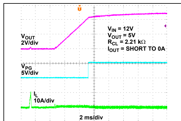
FIGURE 2-52: Recovery from Short Circuit.
