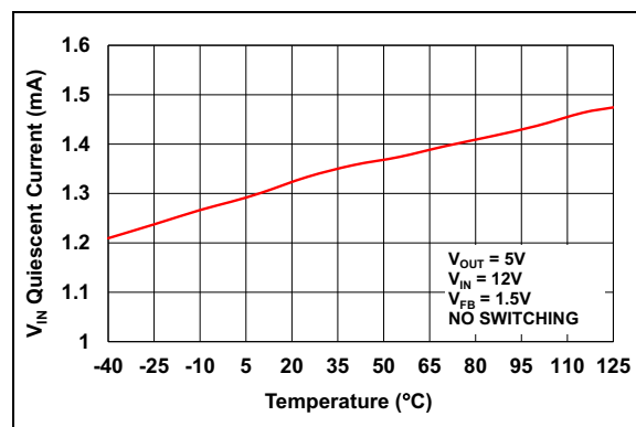
FIGURE 2-16: V_{IN} Quiescent Current vs. Temperature.
