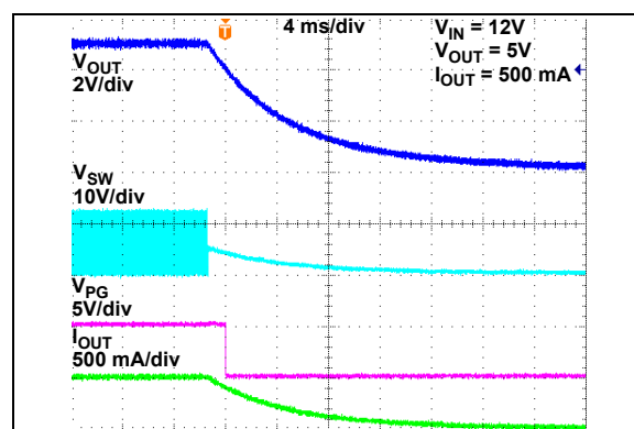
FIGURE 2-53: Behavior when Entering Thermal Shutdown.
