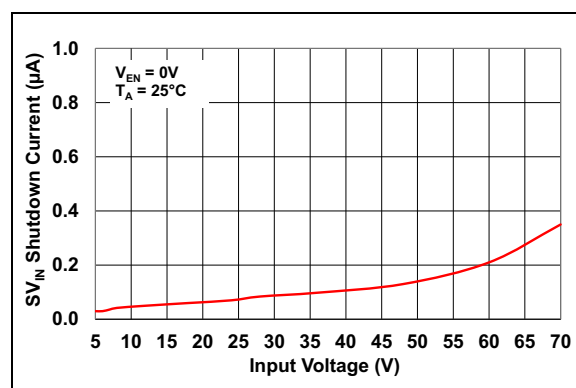
FIGURE 2-29: SV_{IN} Shutdown Current vs. Input Voltage.
