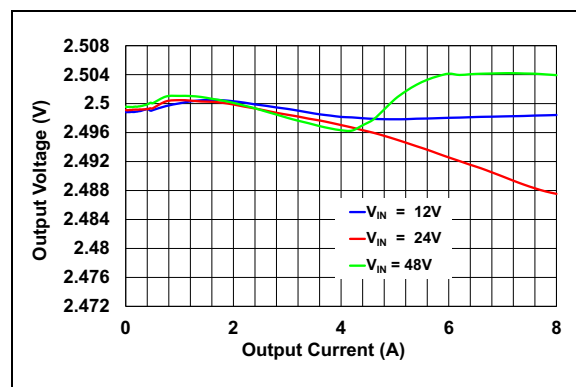
FIGURE 2-5: Output Voltage vs. Output Current ( V_{OUT} = 2.5V ).
