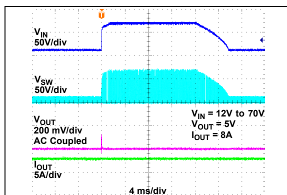
FIGURE 2-65: Line Transient Response ( V_{IN} = 12V to 70V ).
