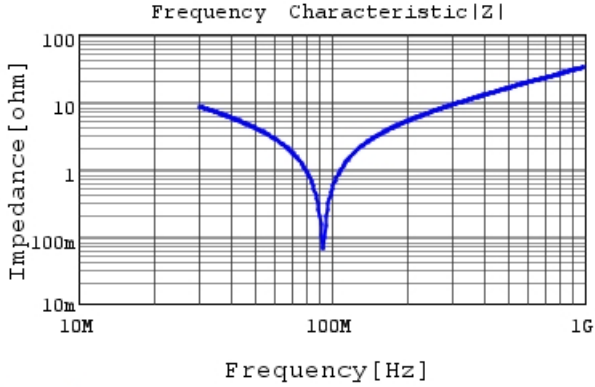
RCE5C2E561J1K1H03B |Z| DC0V, 25degC
