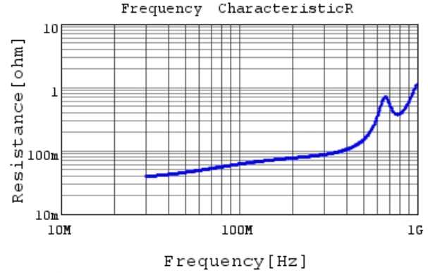
RCE5C2E561J1K1H03B R DC0V, 25degC
