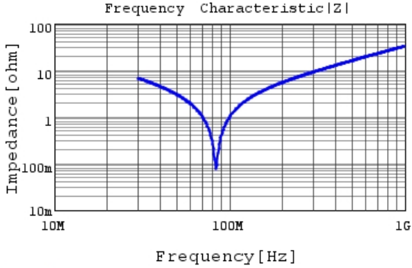
RCE5C2E681J1K1H03B |Z| DC0V,25degC
