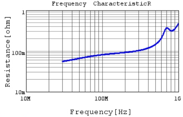
RCE5C2E681J1K1H03B R DC0V,25degC
