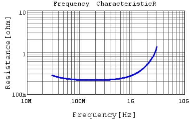
RDE5C2J470J1K1H03B R DC0V, 25degC
