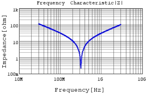
RDE5C2J470J1K1H03B |Z| DC0V, 25degC
