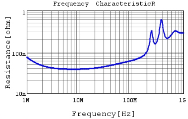
RCE5C2E332J1K1H03B R DC0V, 25degC
