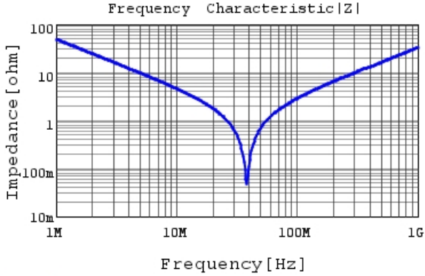
RCE5C2E332J1K1H03B |Z| DC0V, 25degC
