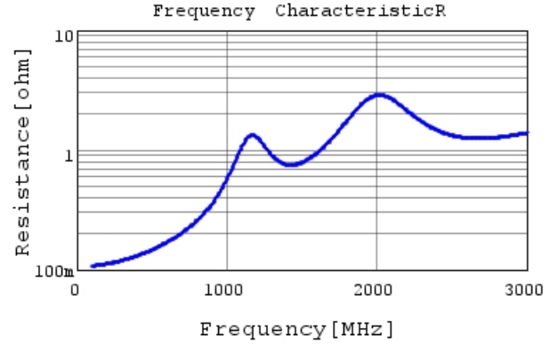
GRM31A7U2J181JW31 R DC0V, 25degC
