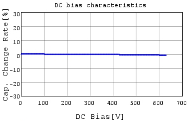
GRM31A7U2J181JW31 C-DC bias capchange, 25.0c
