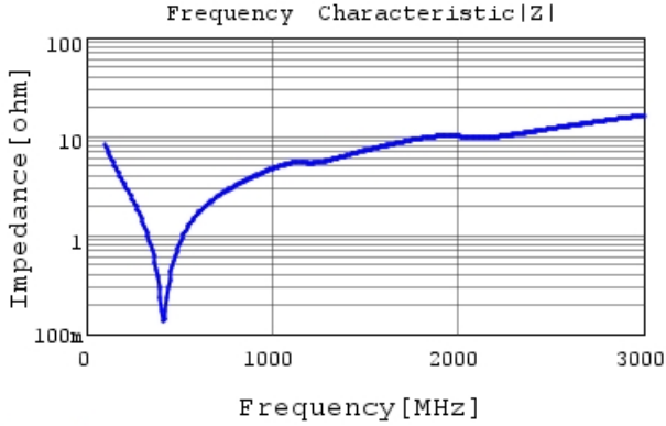
GRM31A7U2J181JW31 |Z| DC0V, 25degC
