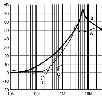
FN 22-0.8/3 types
