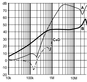
20 amp types
