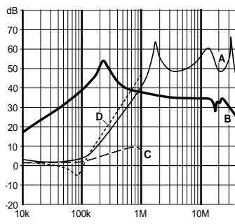
FN 22-0.8/2 types
