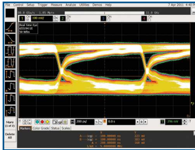
Figure 4. Eye diagram with no correction, notice the minimized eye margins due to fixture loss
