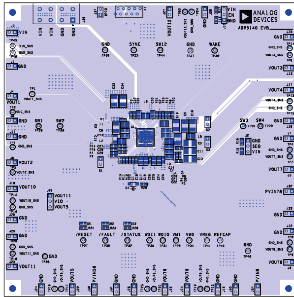
Figure 10. Layer 1, Component Side
