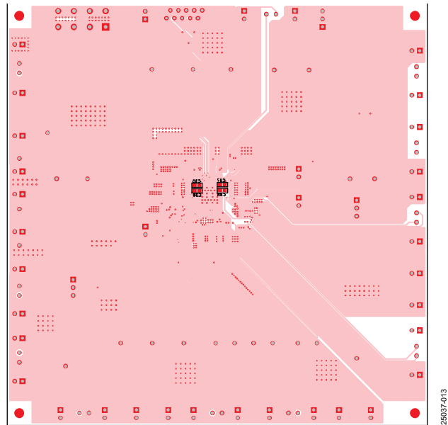
Figure 13. Layer 4, Bottom Side
