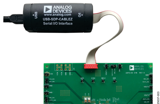
Figure 3. USB-SDP-CABLEZ Connection
