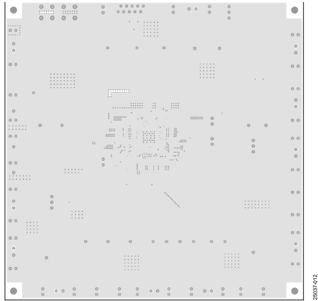
Figure 12. Layer 2, Ground Plane
