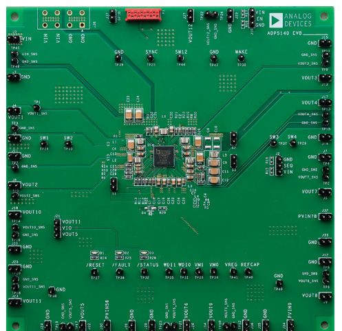
Figure 1. ADP5140-EVALZ Evaluation Board
