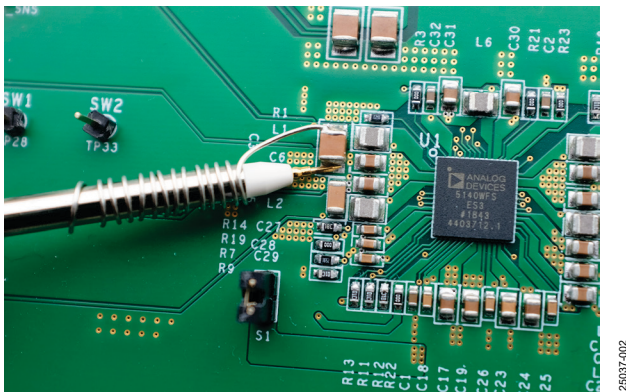
Figure 2. Measuring Output Voltage Ripple
