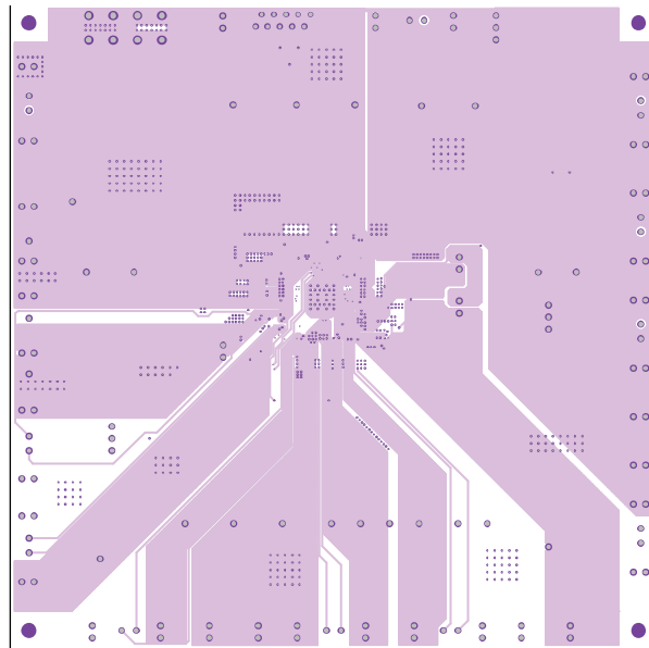
Figure 11. Layer 3, Power Plane
