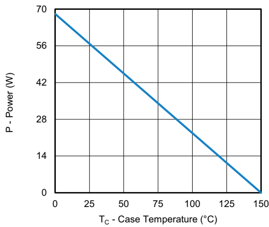
Power, Junction-to-Case
