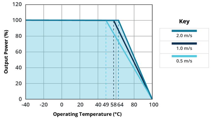
TEMPERATURE DERATING CURVE ( V_{in} = 48V ) PQA100-48-S24-O
