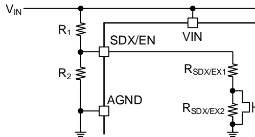
Figure 46. Position of Resistors Connected to the SDX/EN Pin
