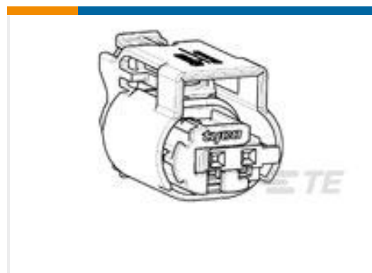
TE Part #1-1438608-5 2POS MQS REC SEALED COD A
