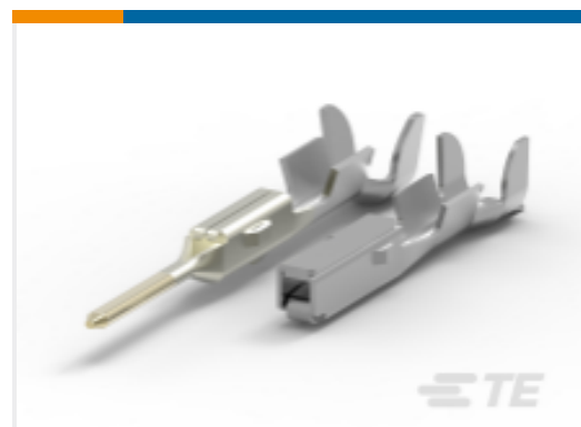
TE Part #284088-1 MULTILOCK, RECEPTACLE AND TAB
