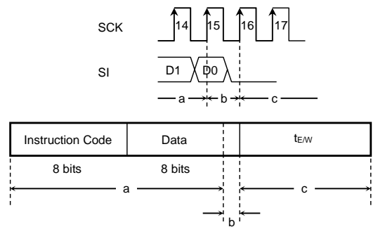
Figure 56. WRSR Cancel Valid Timing
