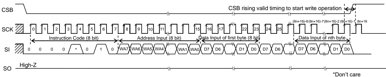
Figure 44. Write Command (Page Write)
