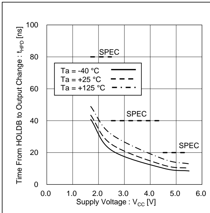
Figure 33. Time from HOLD to Output Change vs Supply Voltage
