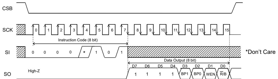
Figure 46. Read Status Register Command
