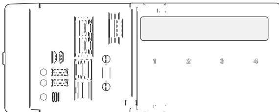
Figure 24. cRIO-9035/9036/9037/9038/9039 Front Dimensions
