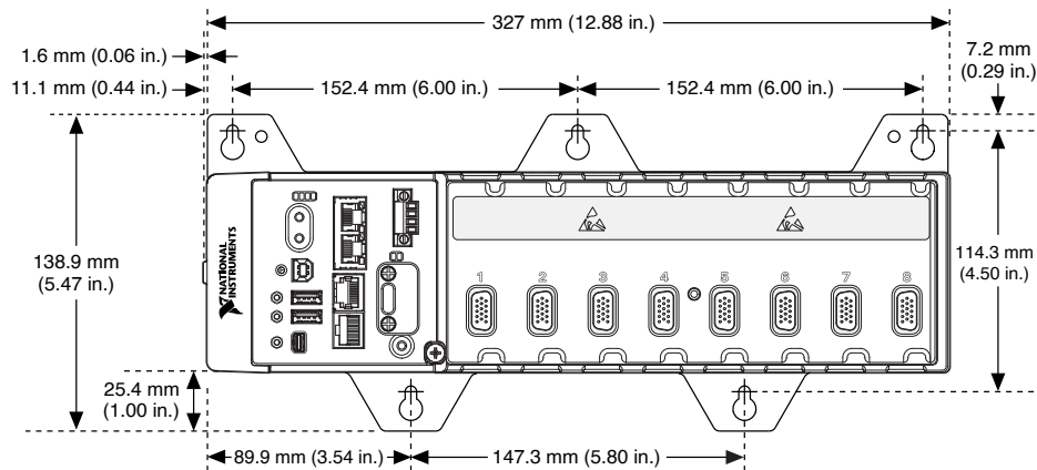
Figure 34. cRIO-9035/9036/9037/9038/9039 Panel Mounting Dimensions
