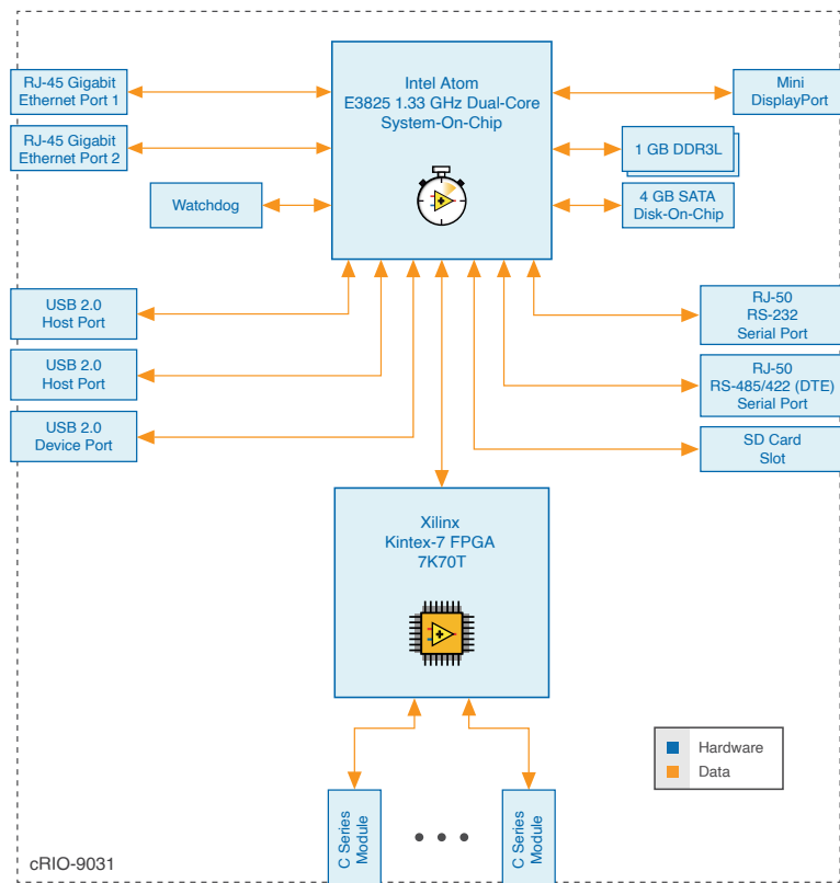
Figure 42. cRIO-9031 Block Diagram
