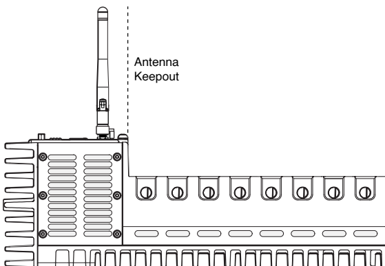
Figure 7. Antenna Keepout
