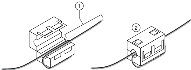
Figure 14. Installing a Ferrite on the Power Leads
