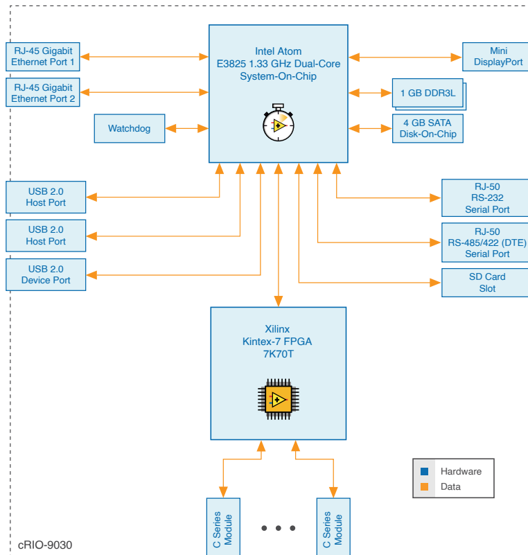
Figure 41. cRIO-9030 Block Diagram
