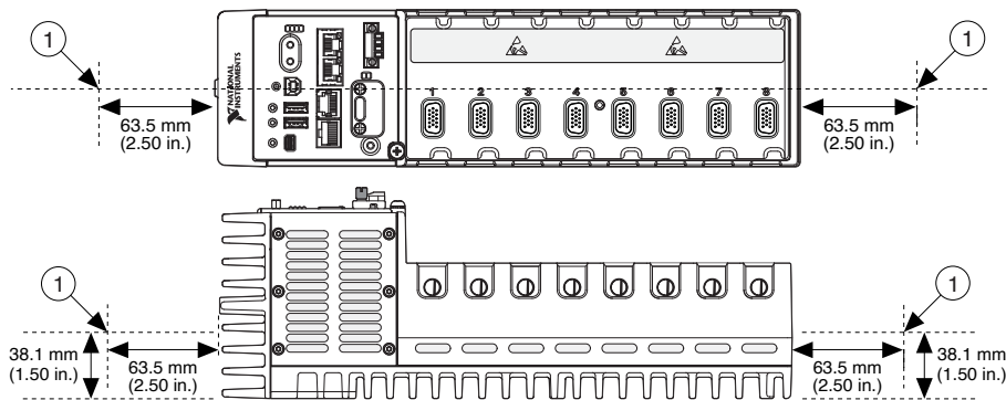
Figure 22. cRIO-903x Ambient Temperature Location
