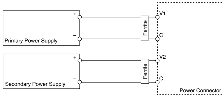
Figure 15. Power Connections
