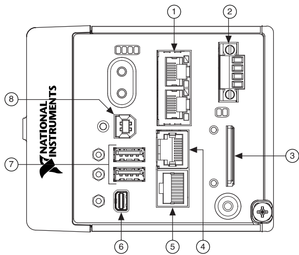
Figure 8. cRIO-9030/9031/9033/9034/9035/9036/9038/9039 Ports and Connectors
