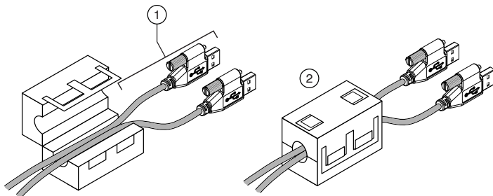
Figure 16. Installing a Ferrite on the USB Cables
