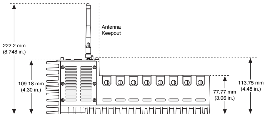
Figure 25. cRIO-9032/9037 Antenna Dimensions
