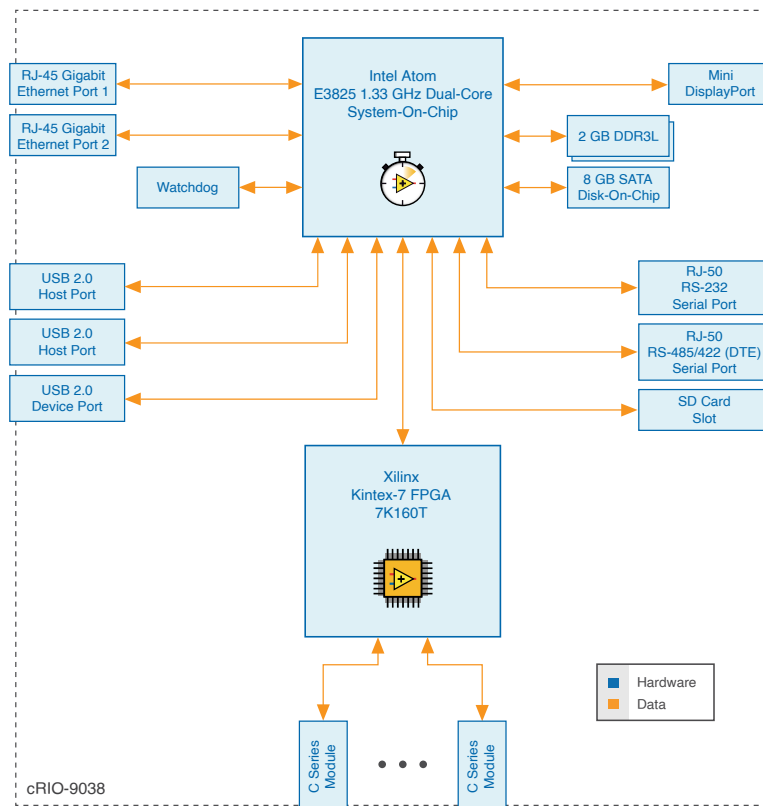
Figure 49. cRIO-9038 Block Diagram
