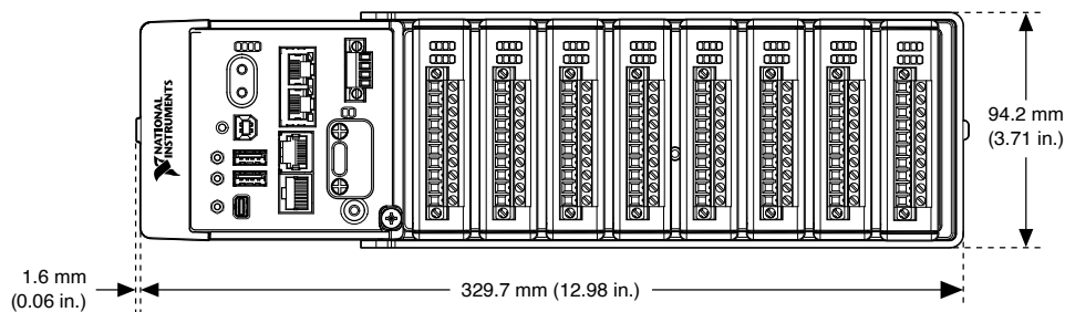
Figure 18. cRIO-9035/9036/9037/9038/9039 Module Immobilization Accessory Dimensions
