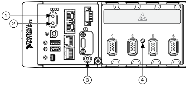
Figure 8. cRIO-9030/9031/9033/9034/9035/9036/9038/9039 Buttons
