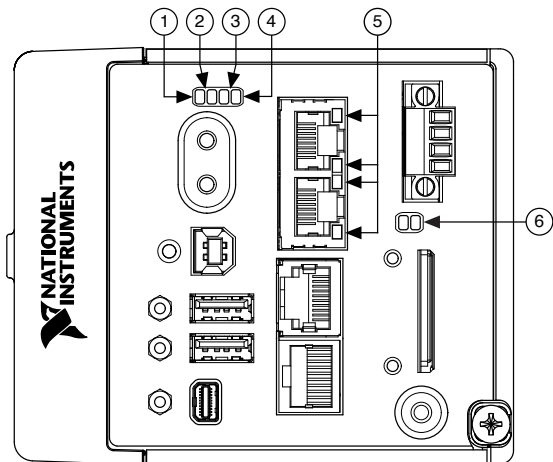
Figure 11. cRIO-9030/9031/9033/9034/9035/9036/9038/9039 LEDs
