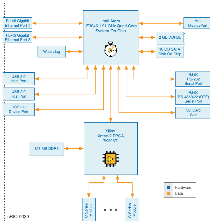
Figure 50. cRIO-9039 Block Diagram
