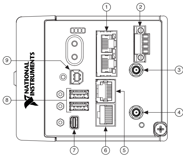
Figure 6. cRIO-9032/9037 Ports and Connectors
