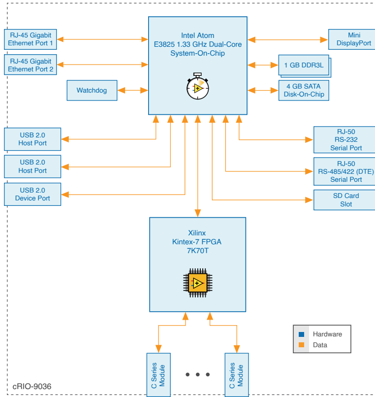
Figure 47. cRIO-9036 Block Diagram
