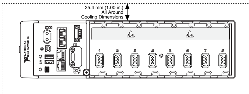
Figure 20. cRIO-903x Cooling Dimensions
