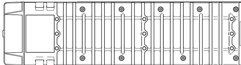
Figure 30. cRIO-9035/9036/9037/9038/9038 Surface Mounting Dimensions
