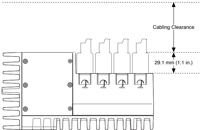
Figure 21. cRIO-903x Cabling Clearance
