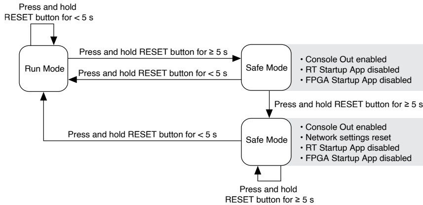
Figure 10. Reset Button Behavior
