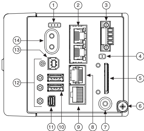
Figure 3. cRIO-9030/9031/9033/9034/9035/9036/9038/9039 Front Panel
