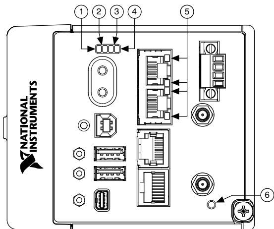
Figure 12. cRIO-9032/9037 LEDs
