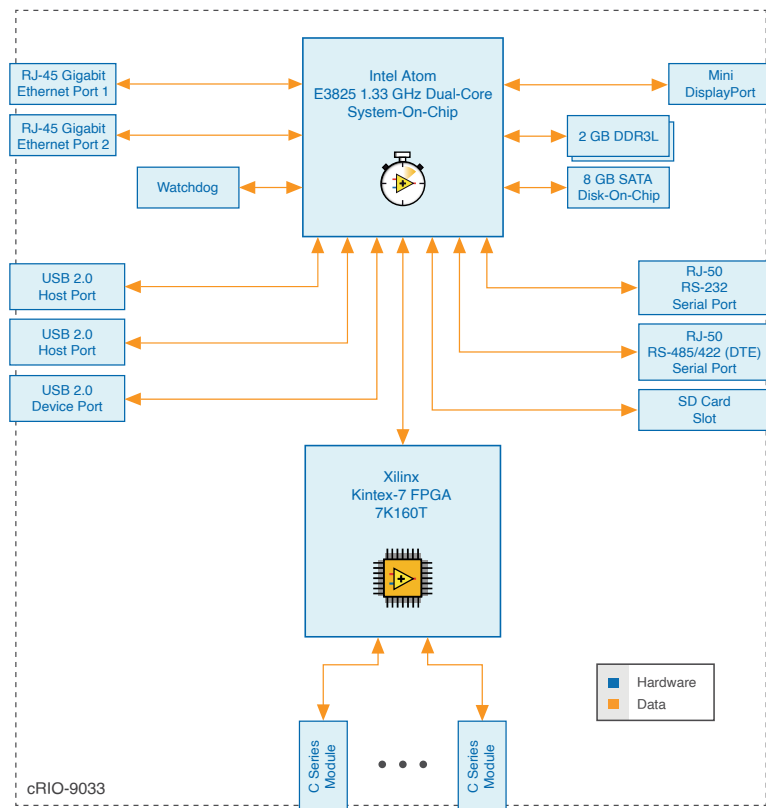
Figure 44. cRIO-9033 Block Diagram
