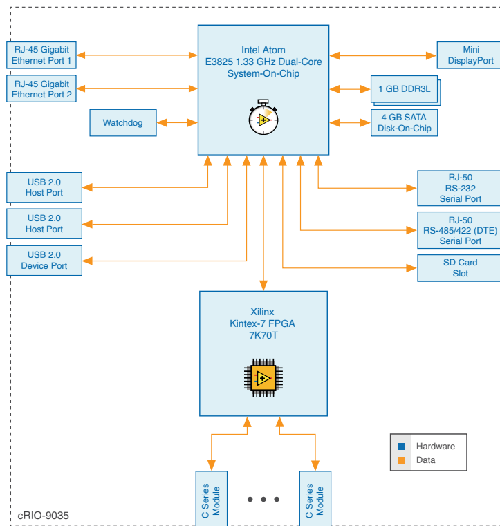
Figure 46. cRIO-9035 Block Diagram
