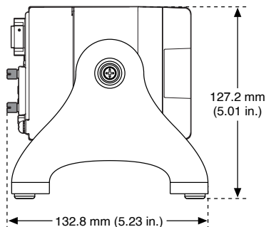
Figure 40. cRIO-903x Desktop Mounting Side Dimensions
