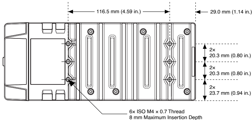
Figure 30. cRIO-9035/9036/9037/9038/9038 Surface Mounting Dimensions
