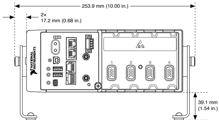
Figure 39. cRIO-9035/9036/9037/9038/9039 Desktop Mounting Front Dimensions
