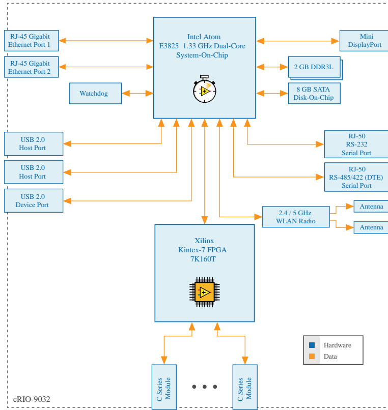
Figure 43. cRIO-9032 Block Diagram
