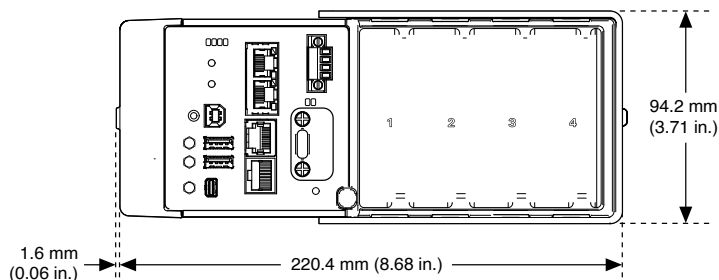
Figure 18. cRIO-9035/9036/9037/9038/9039 Module Immobilization Accessory Dimensions
