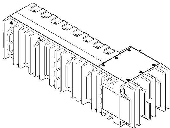
Figure 28. cRIO-9035/9036/9037/9038/9039 Panel Mounting
