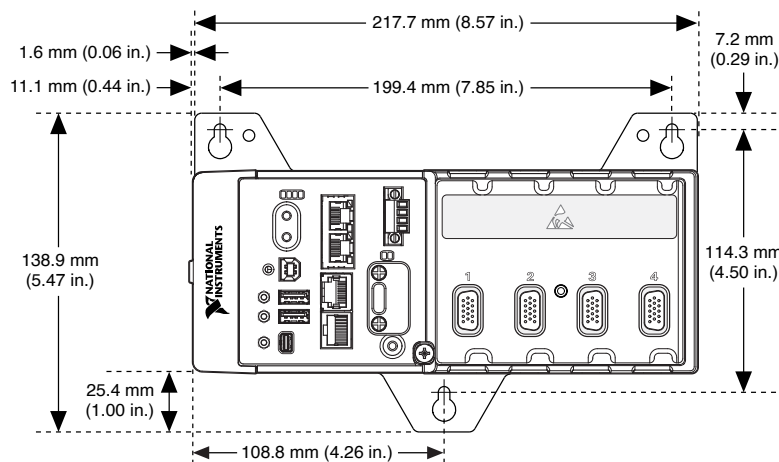
Figure 33. cRIO-9030/9031/9032/9033/9034 Panel Mounting Dimensions
