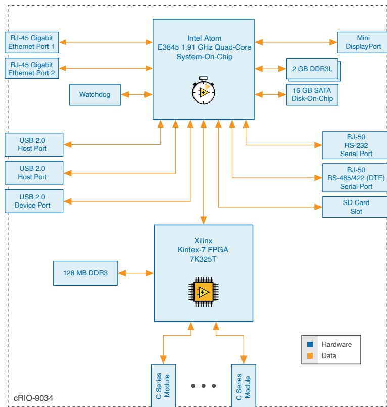
Figure 45. cRIO-9034 Block Diagram
