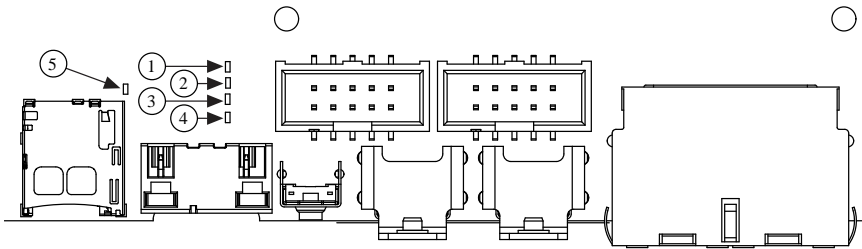
Figure 20. sbRIO-962x/sbRIO-963x LEDs
