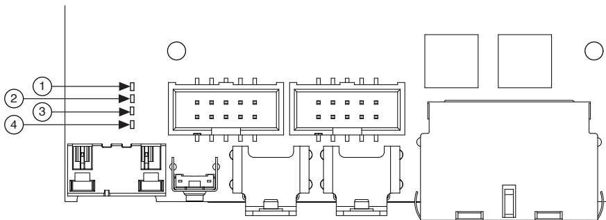
Figure 19. sbRIO-960x LEDs
