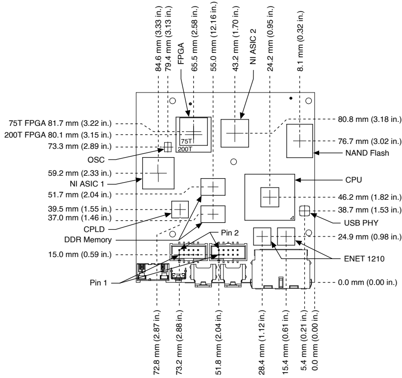
Figure 21. Primary-Side Dimensions
