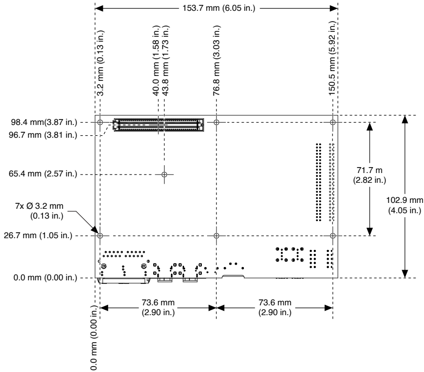
Figure 29. Secondary-Side Dimensions
