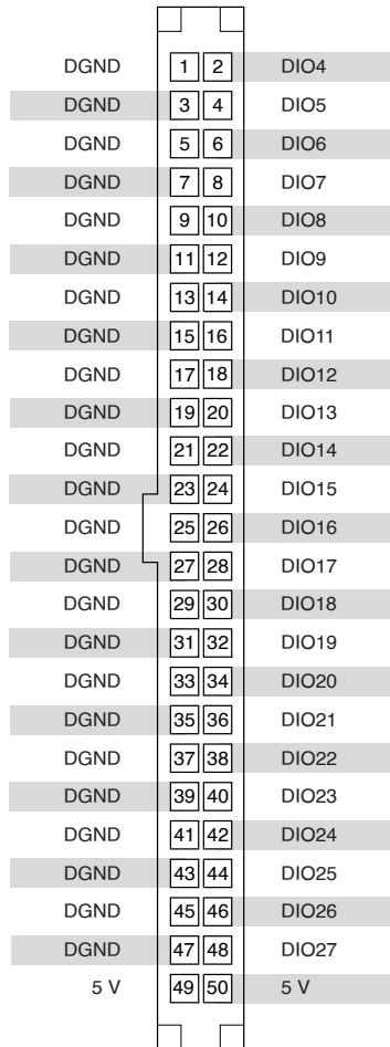
Figure 10. Connector1 Pinout
