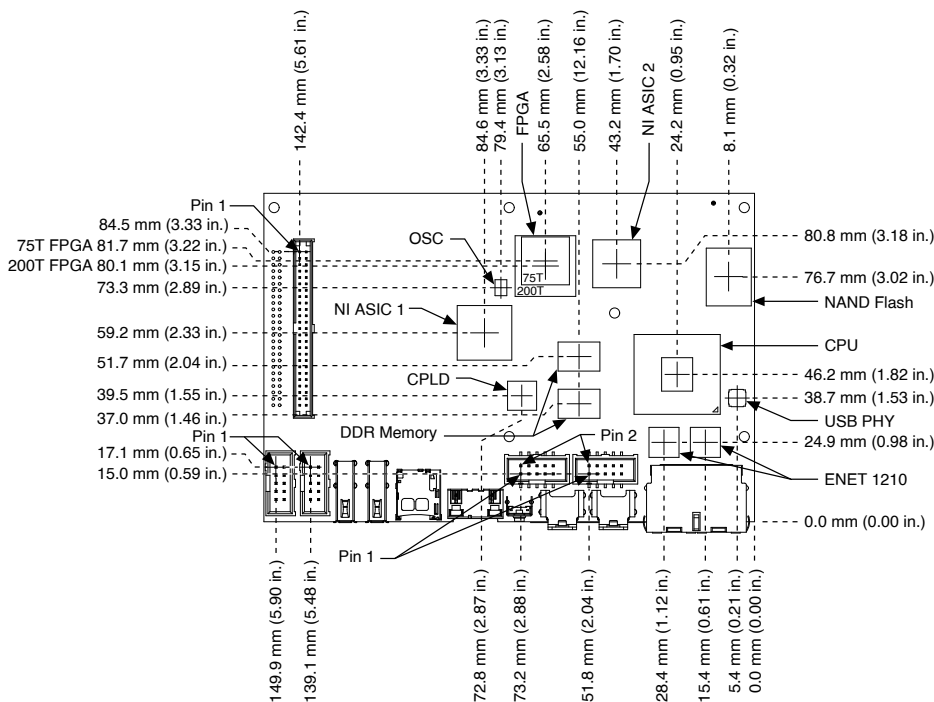
Figure 28. Primary-Side Dimensions
