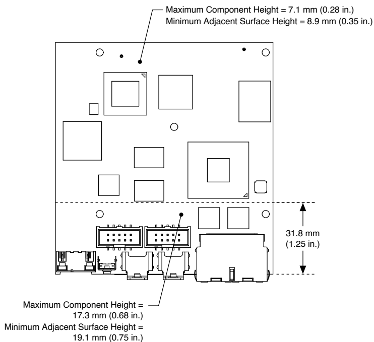
Figure 25. Maximum Component Height of Secondary Side
