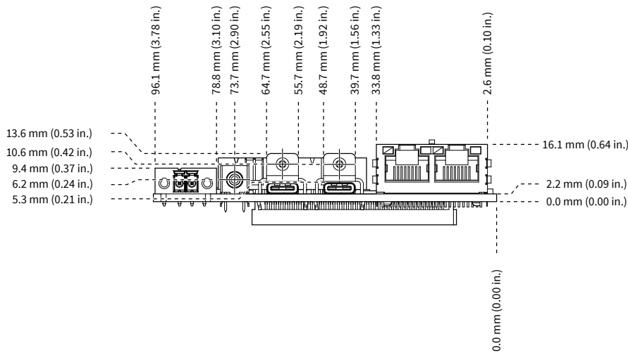
Figure 23. Front Dimensions
