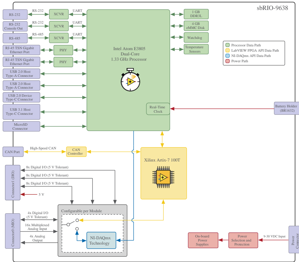
Figure 6. sbRIO-9638 Block Diagram
