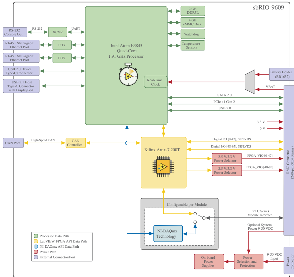
Figure 3. sbRIO-9609 Block Diagram
