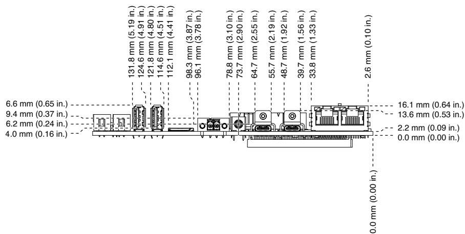
Figure 30. Front Dimensions
