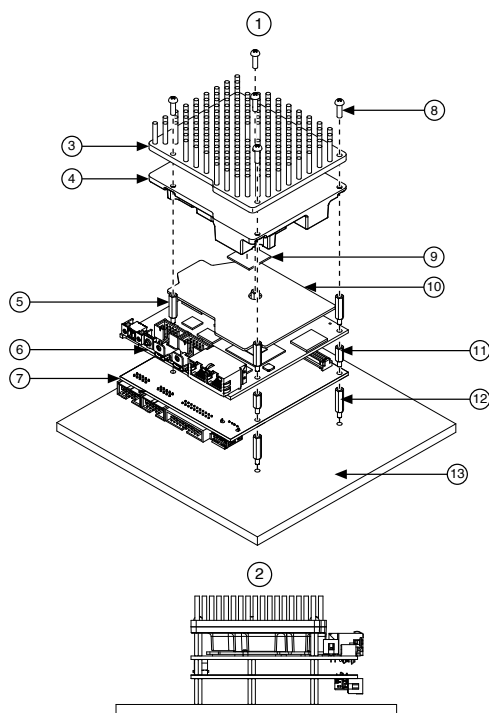
Figure 34. Thermal Convection Mounting
