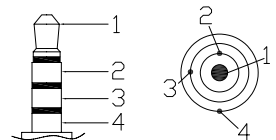
Pin Out Diagram
