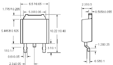
TO-252 Unit: mm
