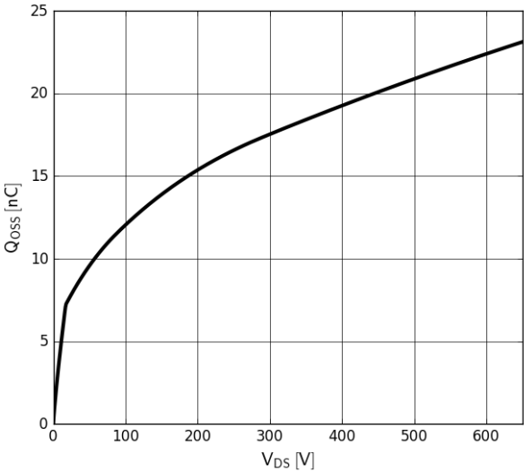
Figure 7. Typical Q_{OSS}
