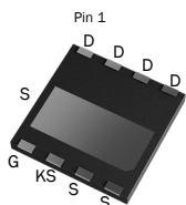
TP65H300G4LSGB PQFN (bottom view)
