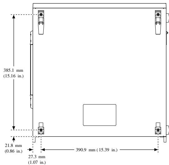
Figure 1. PXIe-1084 Chassis Dimensions (Bottom)
