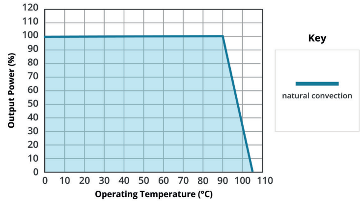
TEMPERATURE DERATING CURVE with heatsink (Vin = 36V)
