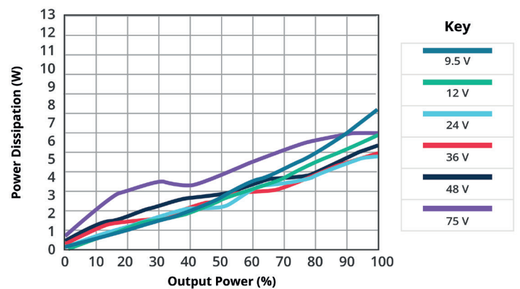
POWER DISSIPATION VS OUTPUT POWER PST50W-36-S15B (at 25°C)
