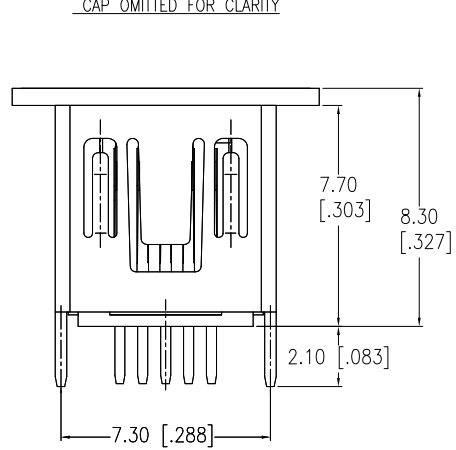
FRONT VIEW ASSEMBLY WITH CAP
