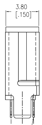
CONTACT TAILS FOR POSITIONS 1, 3 & 5 IN THIS ROW
