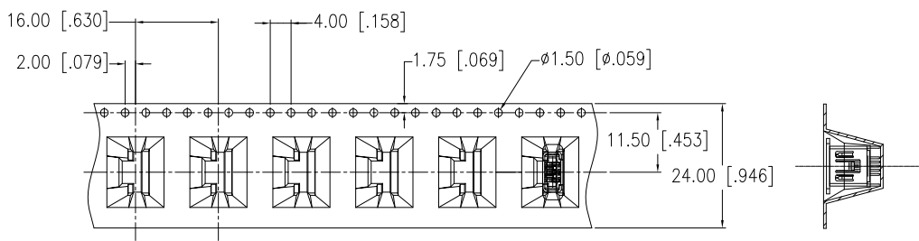
TAPE & REEL LAYOUT
