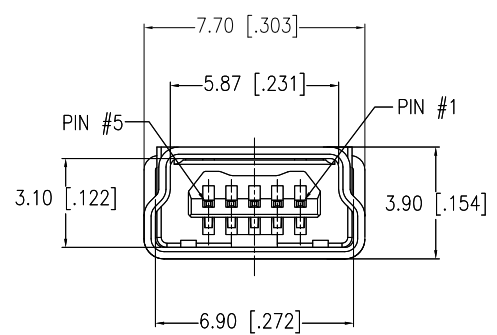
TOP VIEW CAP OMITTED FOR CLARITY
