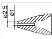
N61-08 Nozzle Standard type Size Φ1.0
