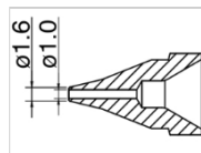
N61-03 Nozzle SS type Size Φ1.0
