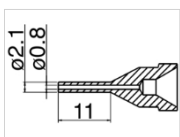
N61-11 Nozzle Long type Size Φ0.8
