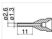
N61-13 Nozzle Long type Size Φ1.3
