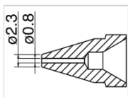
N61-07 Nozzle Standard type Size Φ0.8
