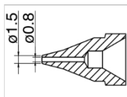
N61-02 Nozzle SS type Size Φ0.8
