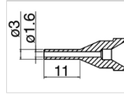
N61-14 Nozzle Long type Size Φ1.6
