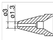
N61-09 Nozzle Standard type Size Φ1.3
