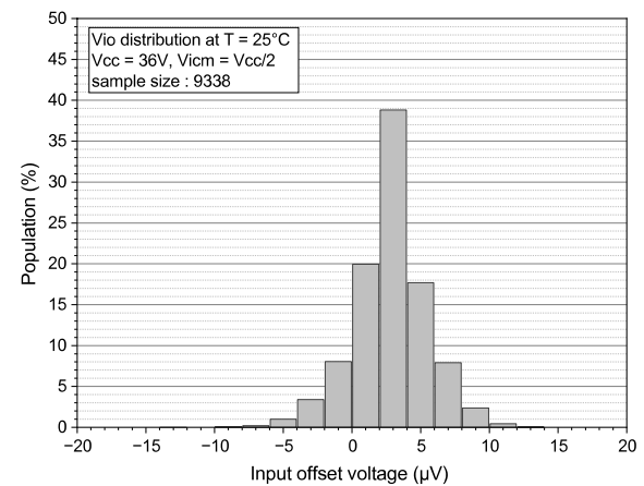
Figure 5. Input offset voltage distribution at V_{CC} = 36\text{ V} and V_{cm} = V_{CC}/2
