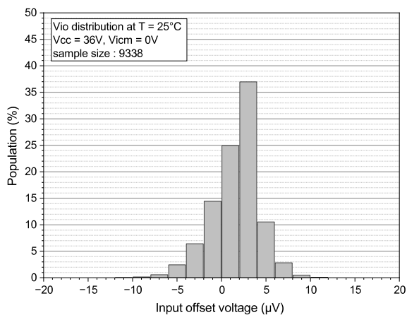
Figure 4. Input offset voltage distribution at V_{CC} = 36\text{ V} and V_{cm} = 0\text{ V}
