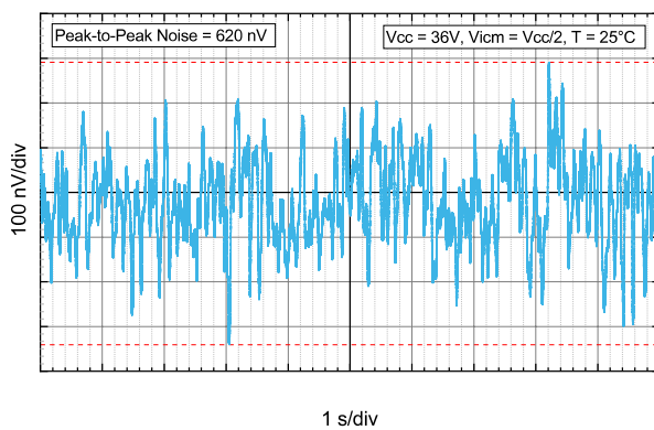
Figure 34. Noise vs. time at V_{CC} = 36\text{ V}
