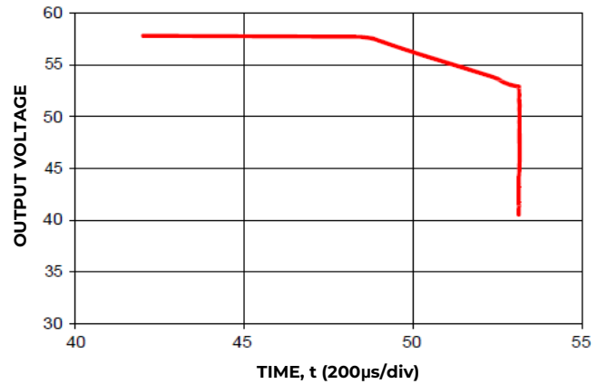
Figure 2. 54V DC output: Power limit, Current limit and shutdown profile at V IN = 185V AC .
