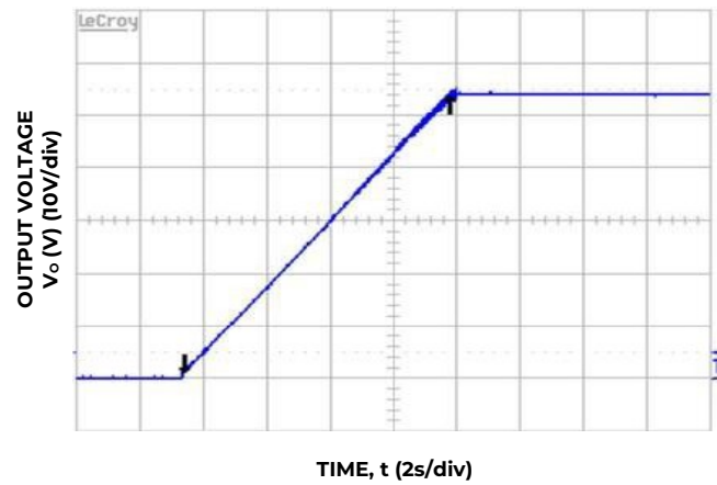
Figure 10. 54V DC soft start, full load, V IN = 185V AC - RS485 mode.
