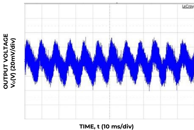
Figure 5. 54V DC output ripple and noise, full load, V IN = 185V AC , 20MHz bandwidth
