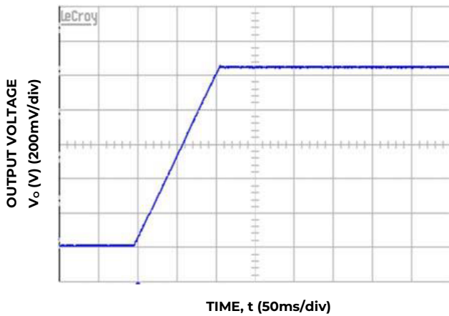
Figure 9. 54V DC soft start, no-load & full load, V IN =185V AC - I 2 C mode.
