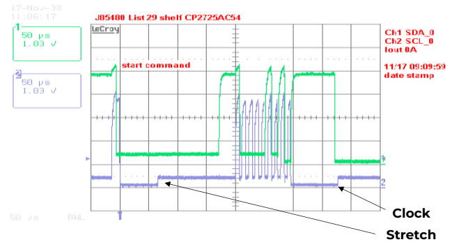
Figure 14. Example waveforms showing clock stretching.
