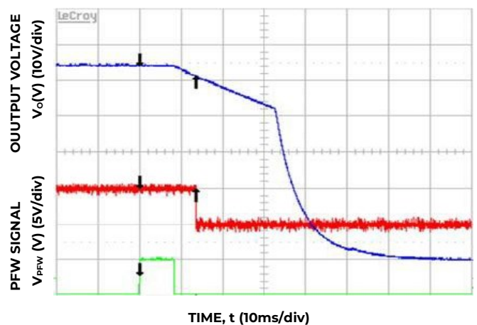
Figure 12. PFW alarmed 19.6ms prior to V O < 40V, output load: 38A, V IN = 185V AC .
