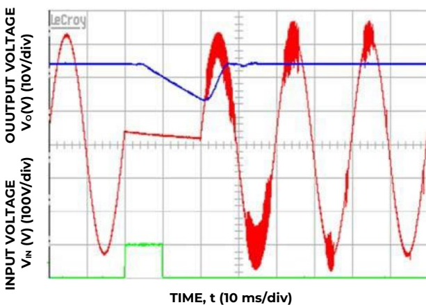
Figure 11. Ride through missing 1 cycle, full load, V IN = 230V AC .
