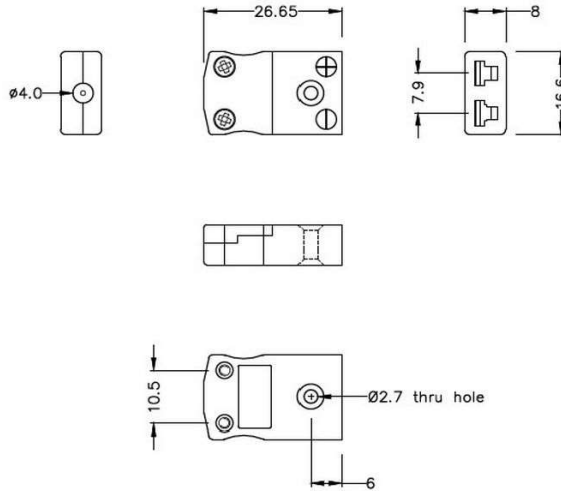
Miniature in-line Socket (dimensions in mm)
