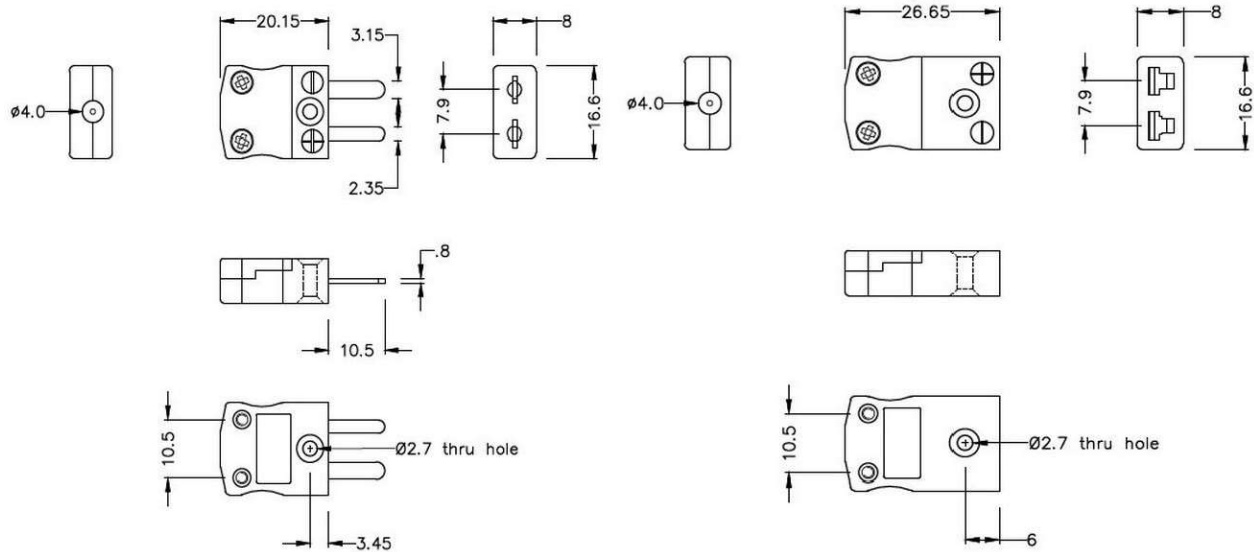
Miniature in-line Socket (dimensions in mm)
