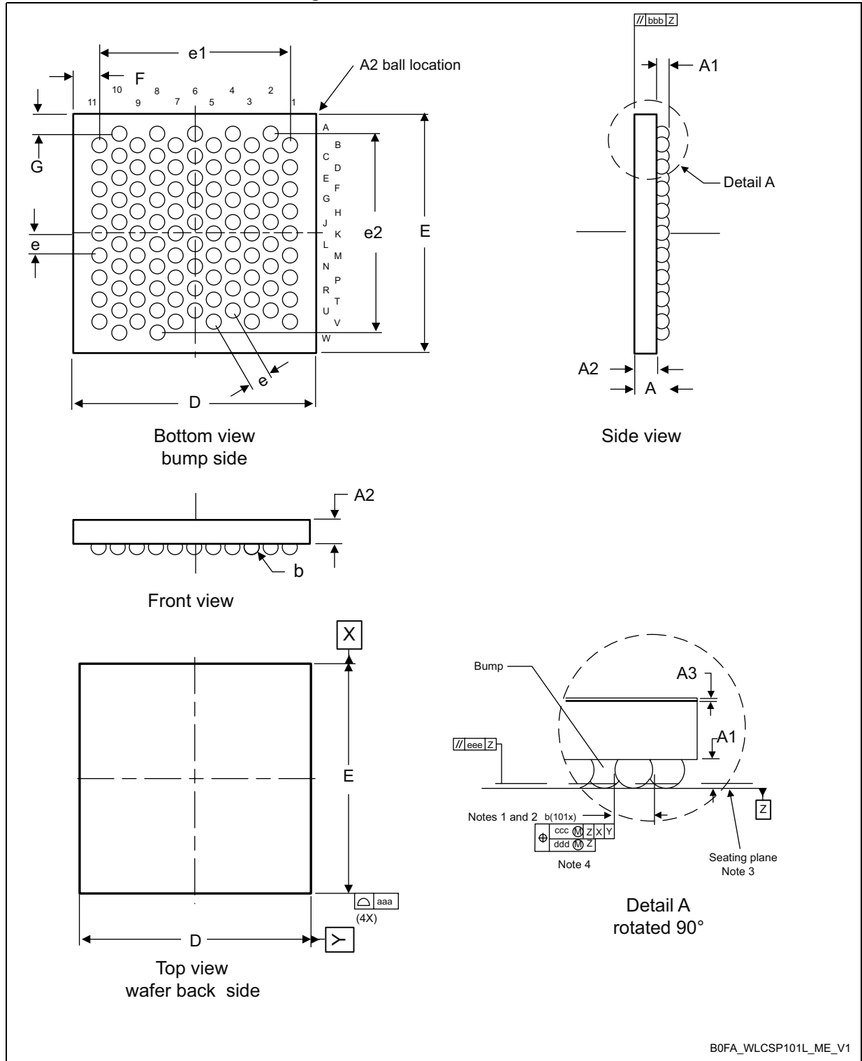
Figure 93. WLCSP101L - Outline
