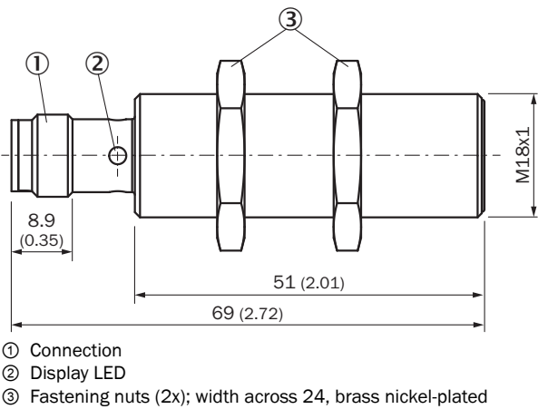
IMS18, V2A, flush
