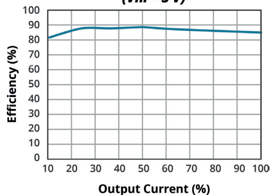
EFFICIENCY VS OUTPUT LOAD PESE2-S5-S5-M (Vin = 5 V)
