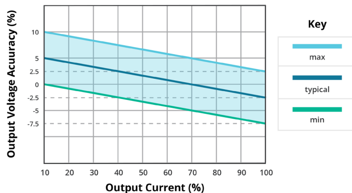
OUTPUT REGULATION CURVE 5 Vdc input model/all other output models (nominal input)
