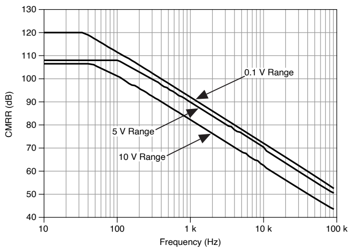
Figure 3. AI <0..15> CMRR
