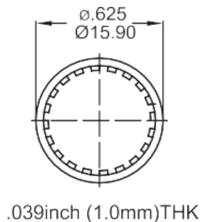
Lockwasher (Std.)
