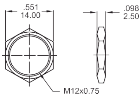
NUT (Std.)
