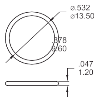
O-Ring (Std.)
