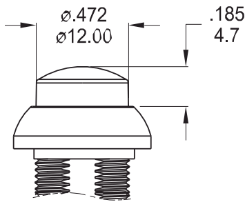
High Raised
