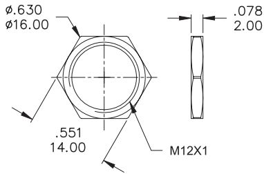
M12x1 NUTS
