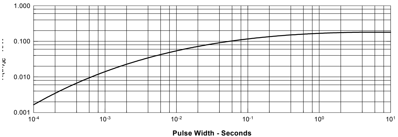
Figure 10. Transient Thermal Resistance
