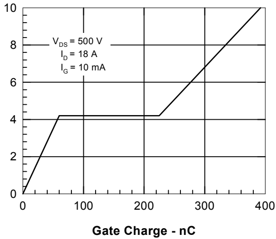
Figure 7. Gate Charge
