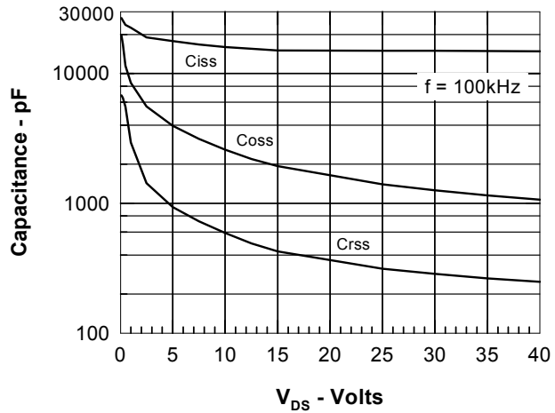
Figure 8. Capacitance Curves
