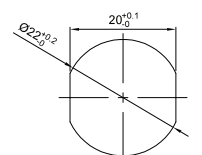
Panel Cutout
