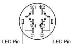
Contact Composition
