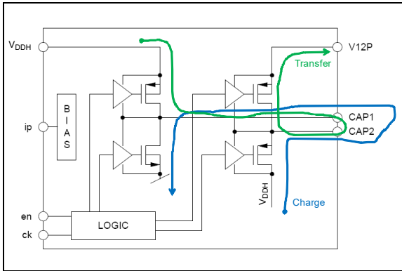
FIGURE 5-1: Charge Pump.
