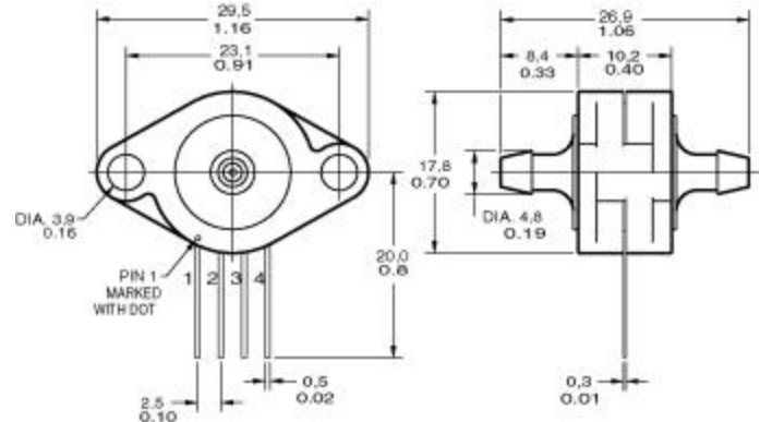
GFS/AFS Housing
