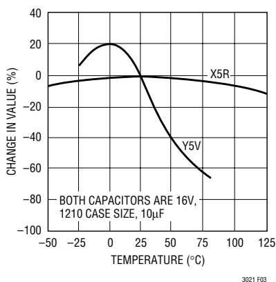
Figure 3. Ceramic Capacitor Temperature Characteristics
