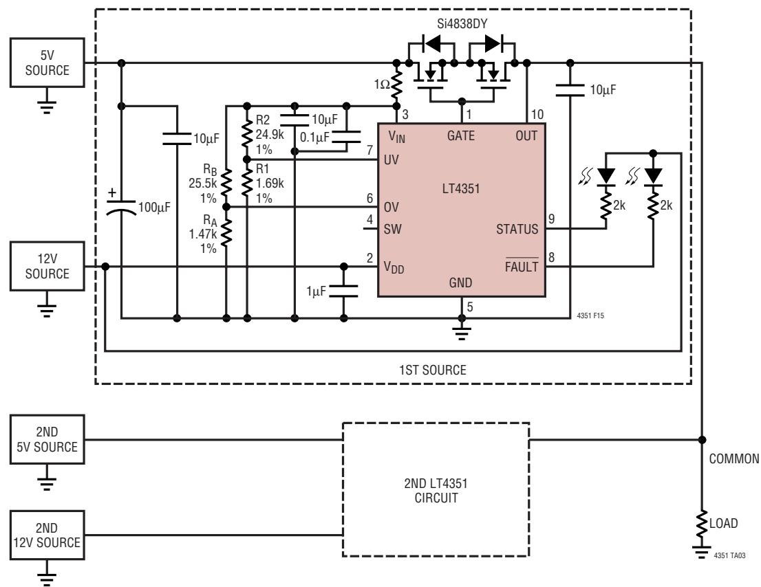
5V Redundant Supply with External V DD
