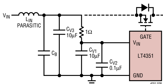
Figure 8. V_{IN} Capacitors
