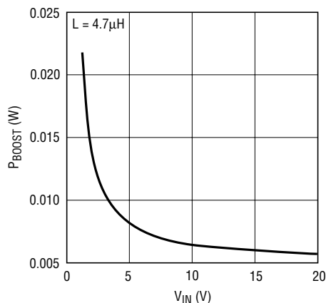
Figure 12. P_{BOOST}(TYP)
