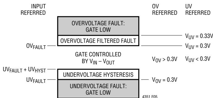
Figure 5. Graphical Representation of the UV and OV Functions
