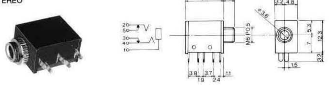
No.MX-238A0 (φ3.5) STEREO
