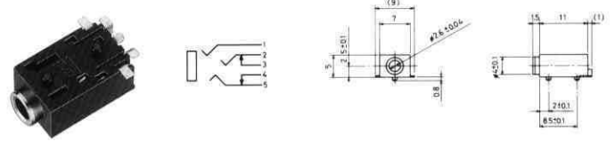
No.MJ-2-348A0 (φ2.5) With Metal Sleeve No.MJ-2-348B0 (φ2.5) Without Metal Sleeve SUB-MINIATURE STEREO JACK
