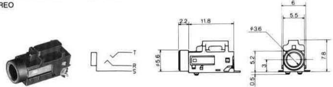
No.MJ-A18 (φ2.5) STEREO
