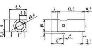
No.MJ-653 3.5MM DOUBLE STEREO JACK FOR P.C. W/FULL SHIELD HOUSING
