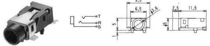
No.M03-292J1 (φ3.5) STEREO
