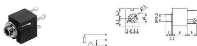
No.MJ-255 (φ2.5) MONO
